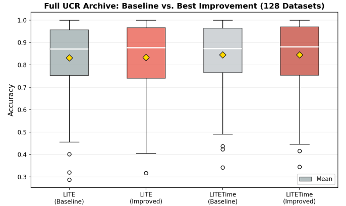
Fig. 10. Accuracy distribution comparison between baseline and improved configurations across the full 128-dataset UCR archive. The improved LITE configuration shows an upward-shifted distribution with a higher median, while LITETime performance remains essentially unchanged. Gold diamonds indicate mean accuracy values.
